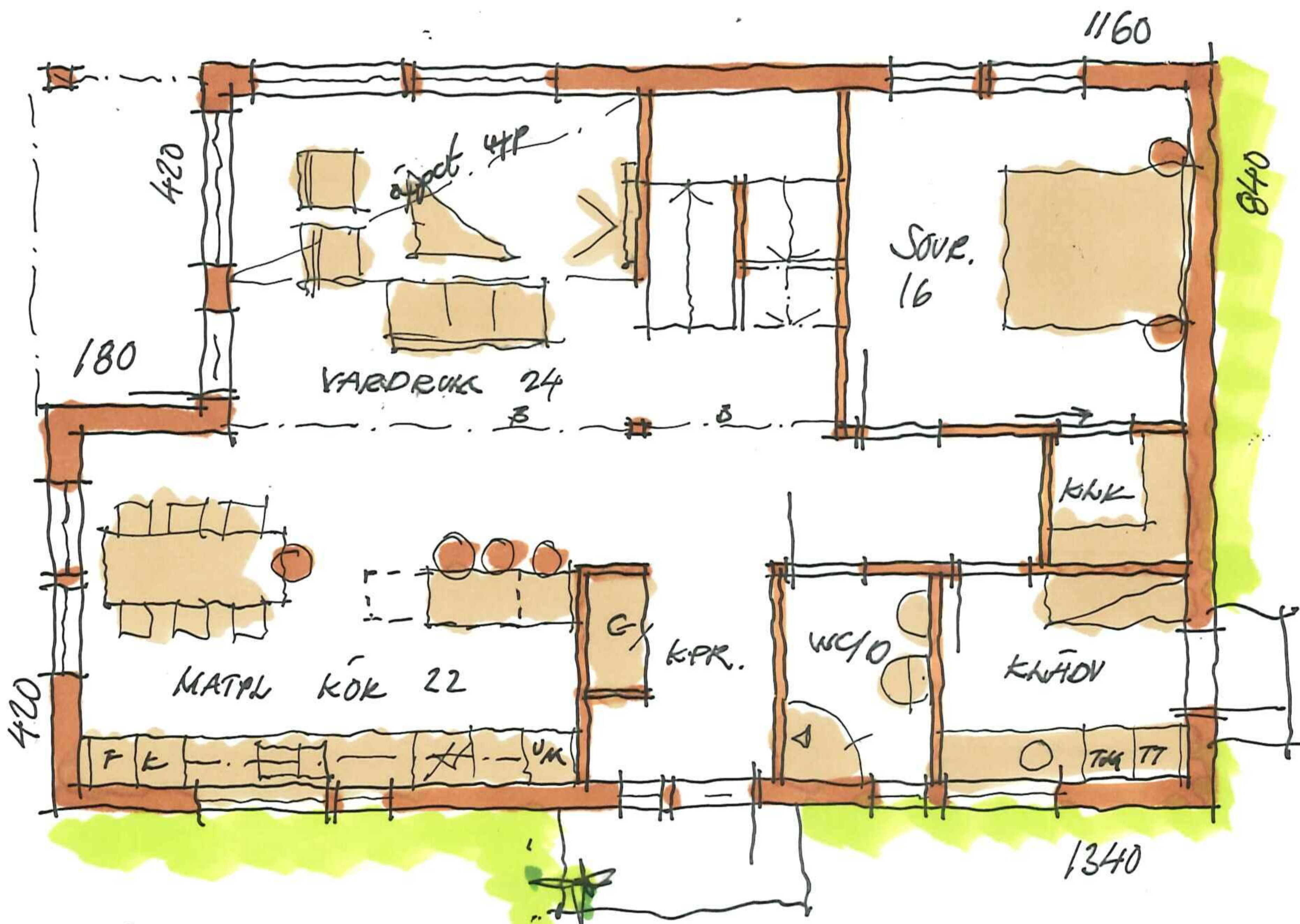
ENTREPLAN BOA 105m 2
